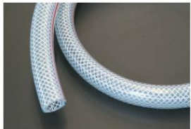
Blow-by hose Part number: 31D003 Size: Inner diameter 15mm, outer diameter 22mm Compatible: L type 2TG, 18RG Price: ¥1,000/1m
