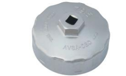
Cup-type oil filter wrench Product number: AVSA-080 Compatible: 18RG Price: ¥2,890 *Filter diameter 80mm
