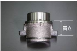
L-type clutch sleeve (Updated 2026.4.6) 16mm ¥4,000 26mm ¥4,430 18mm ¥4,230 28mm ¥2,430 20mm ¥1,830 30mm ¥4,360 22mm ¥1,760 32mm ¥2,360 24mm ¥2,010
