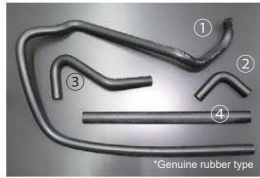
GC110/KHC130 Heater Hose (For early models) *Type where ① and ③ are connected with a heater connector. ① The hose is long, so cut it before use. Price: ¥9,730 /set (Updated 2026.4.16)
