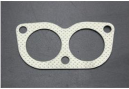
STD Glasses Muffler Gasket Compatible with: GC10/S30 early model *For genuine exhaust Price: ¥800
