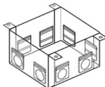
Assembly completed diagram *Stays for fixing are not included
