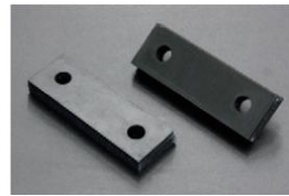
S30, S31 Muffler Hanging Rubber Set *Hole center length 59mm *Board thickness 13mm *Price ¥8,660/2 pcs SET
