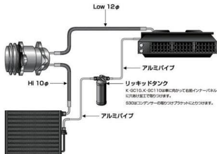
Cooler piping diagram
