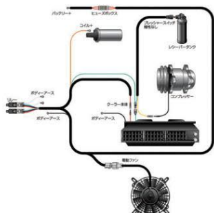
Cooler wiring diagram
