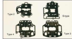
•SOLEX chamber cover gasket 40y S type body ¥550 50y 2 type body ¥550 40y 44y 3 type body ¥550 40y 44y 4 type body ¥550
