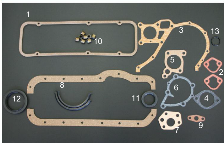
The photo shows the A-type overhaul kit. The above kit does not include the manifold G/K and head G/K.
